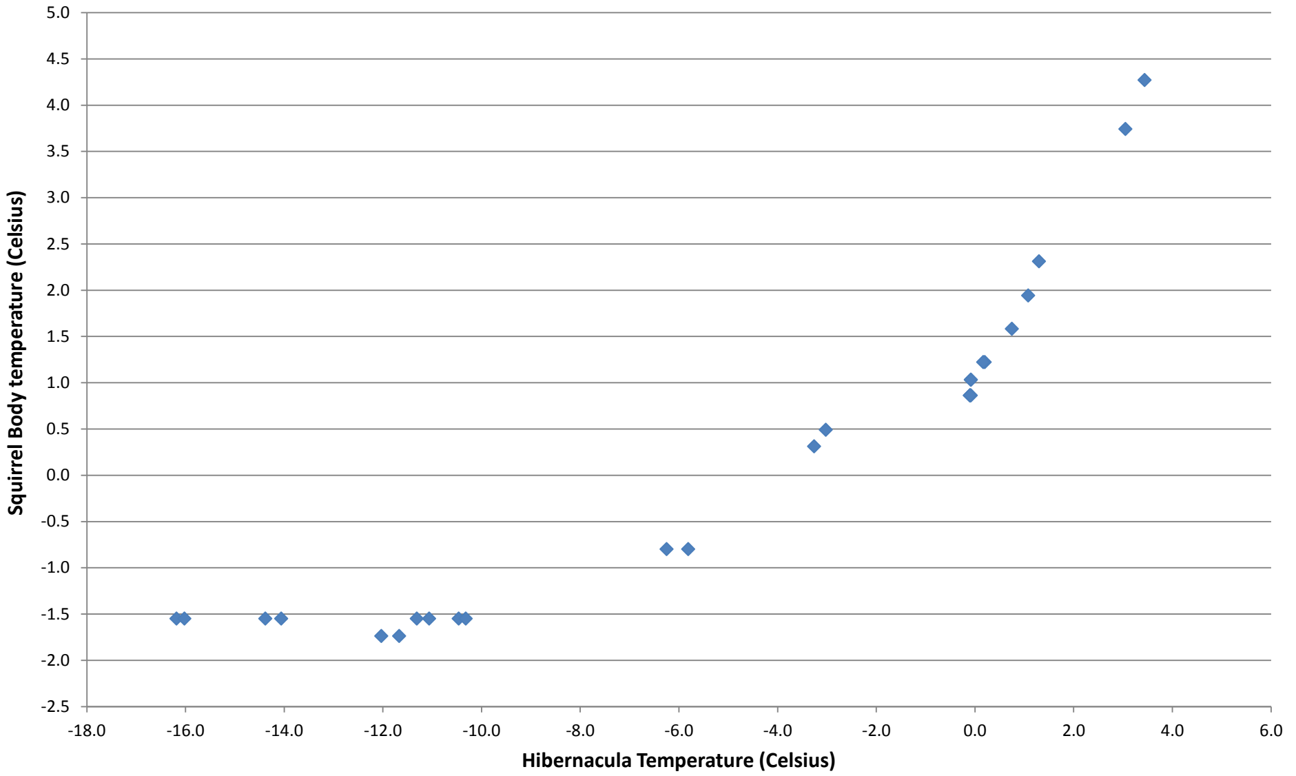
Hibernacula temperature vs Arctic Ground squirrel body temperature during torpor
